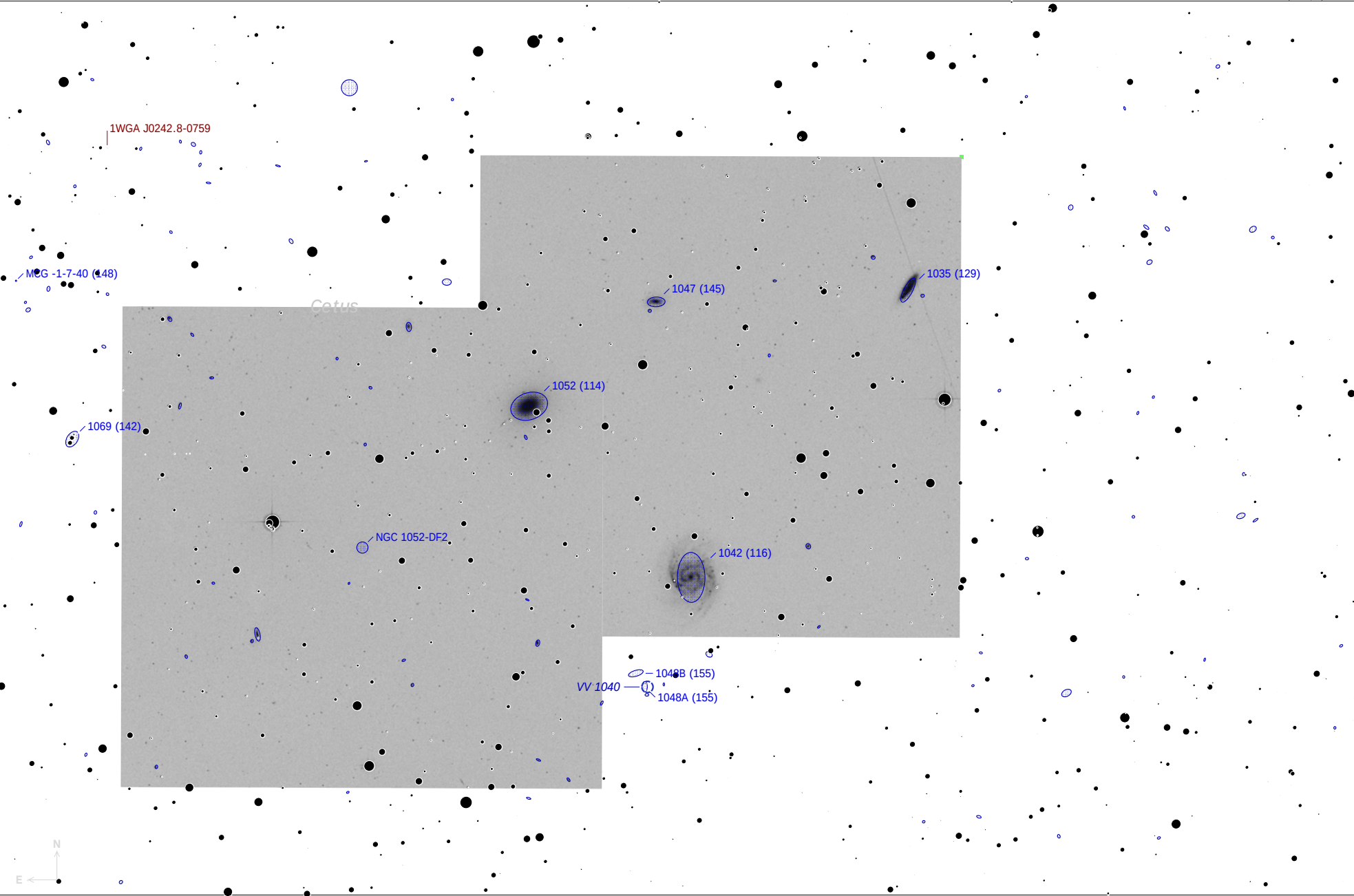
02h40m27.7s -08°17'58" (Skymark) Magnitude: unknown
