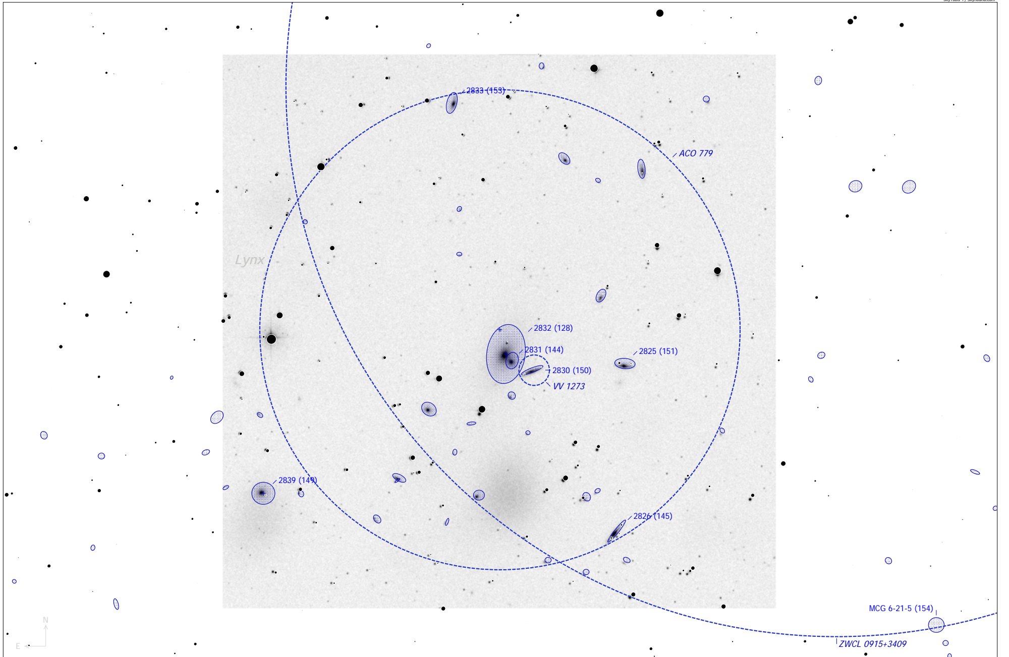
ACO 779 (Galaxy Group) Magnitude: unknown Size: 15.7' Light Time: 0.3 Gyr
